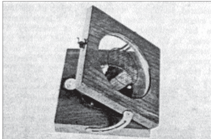
Figure 2 Spherical densiometer, Model B, with estimating grid superimposed between the eye and surface of the concave mirror.
