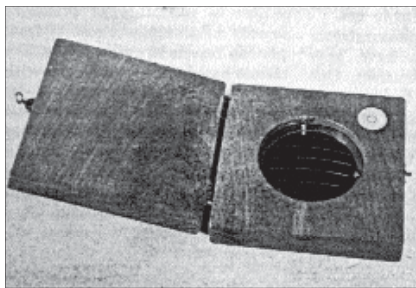
Figure 1 Spherical densiometer, Model A, with estimating grid scratched on the surface of the convex mirror
